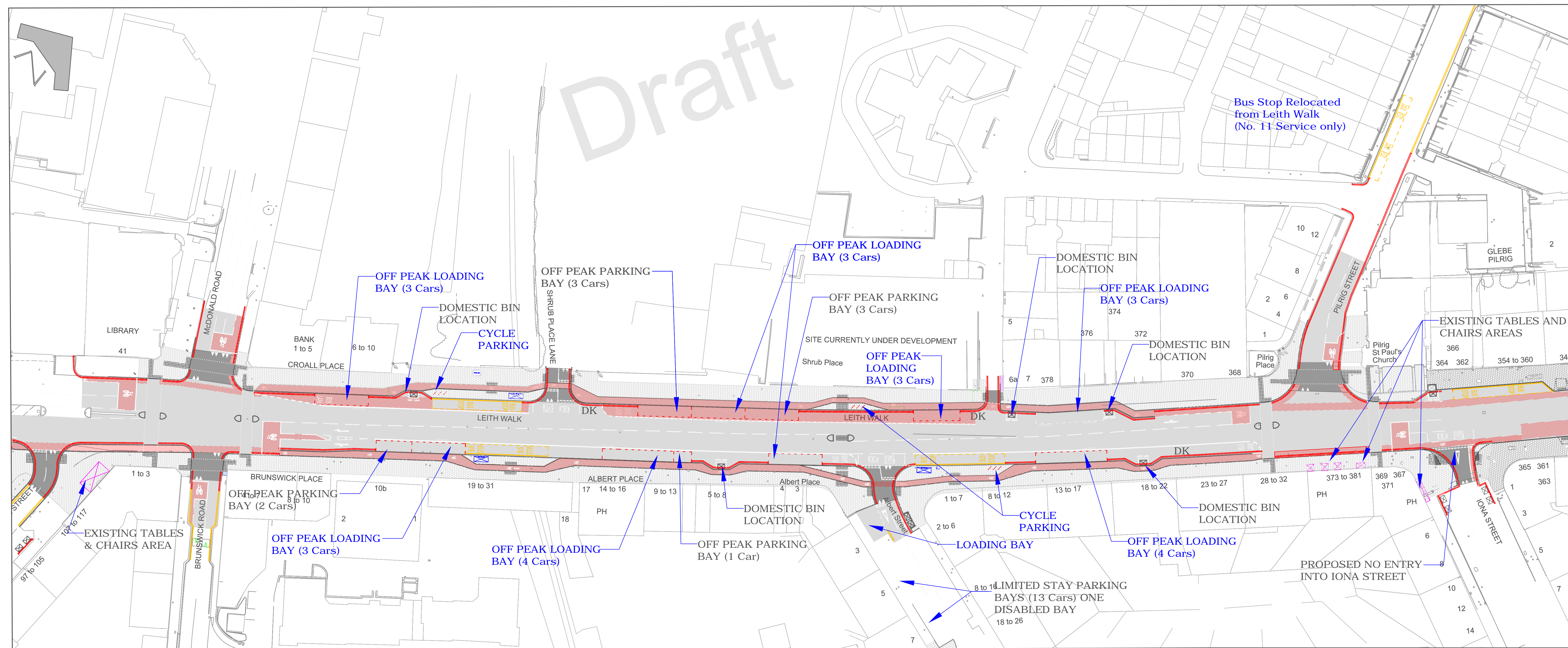
LEITH PROGRAMME DESIGN LAYOUT FOR LEITH WALK BETWEEN McDONALD ROAD AND PILRIG STREET (PHASE 4 - Segregated cycle-way in each direction)
